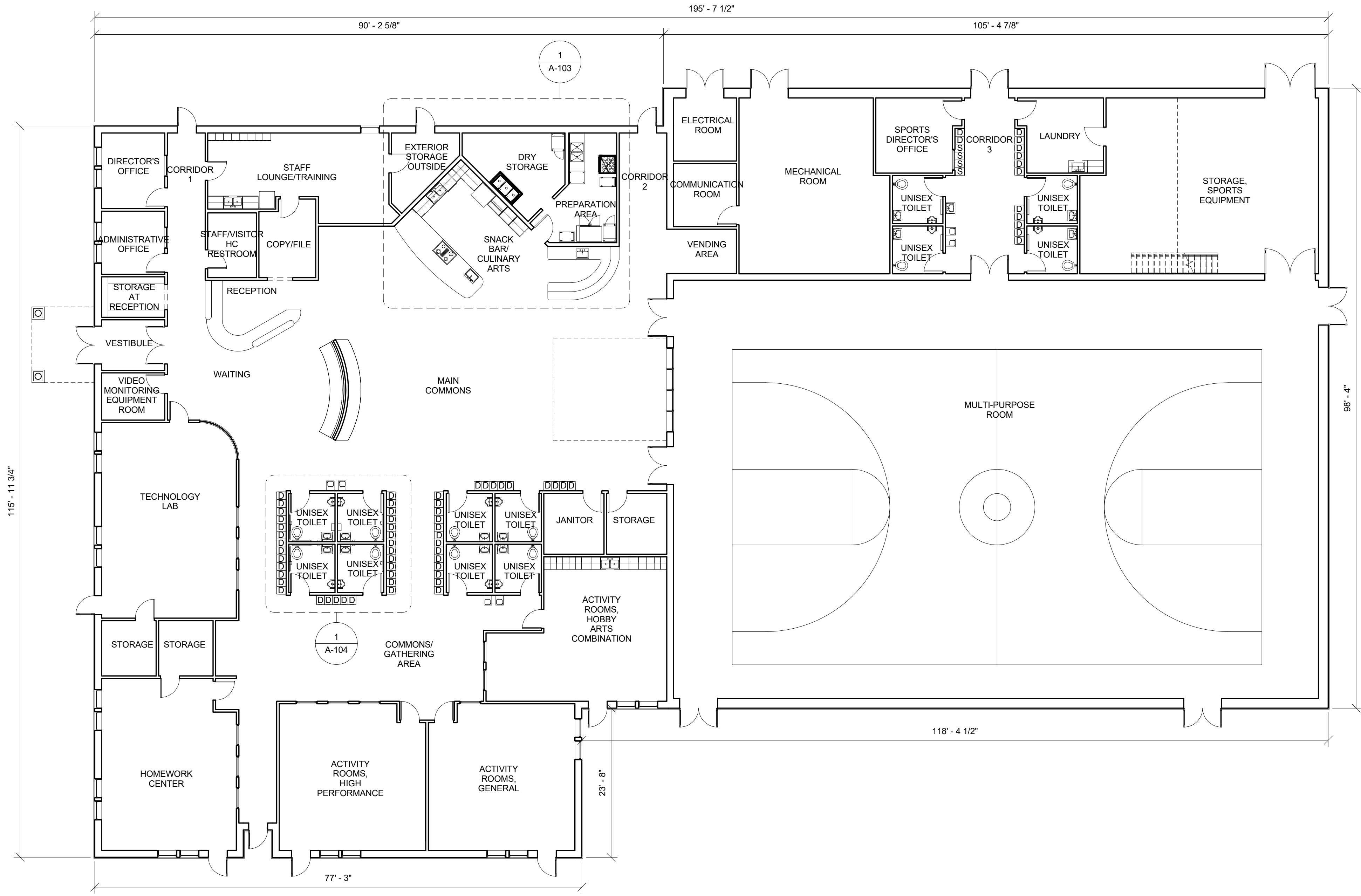
OVERALL FIRST FLOOR PLAN SCALE: 3/32" = 1'-0"
