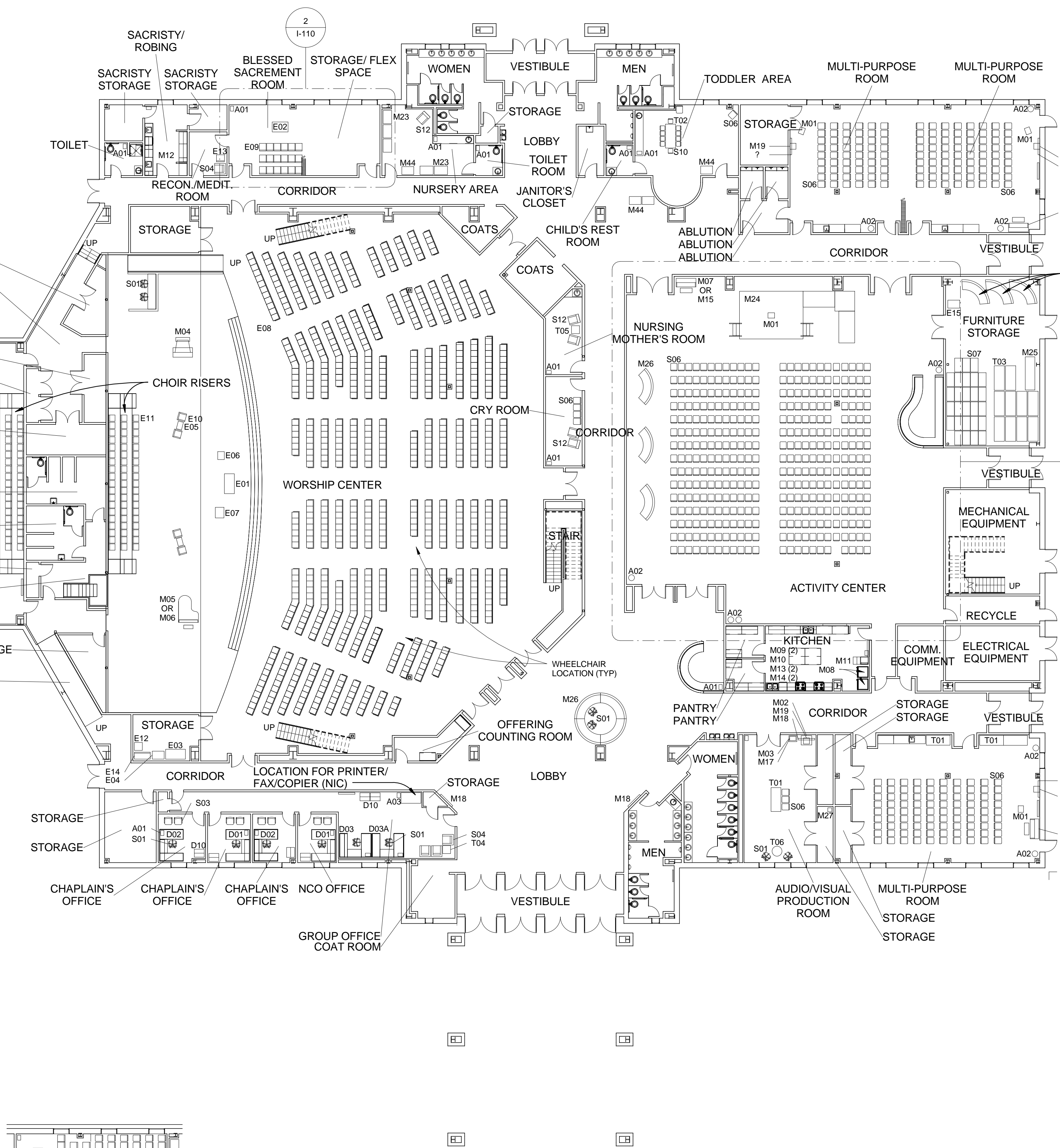
1 COMPOSITE FIRST FLOOR FURNITURE PLAN
