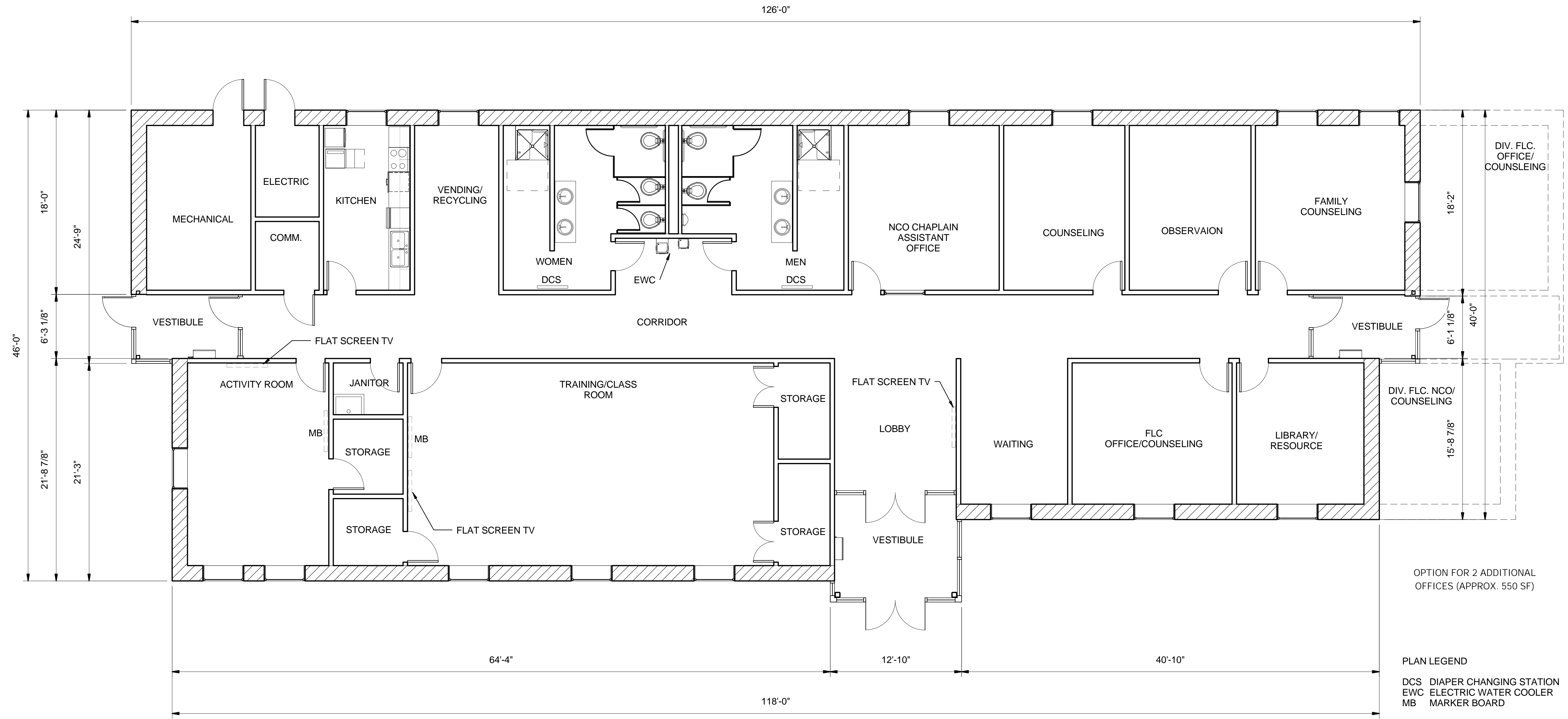
1 COMPOSITE FIRST FLOOR PLAN A-110 3/16" = 1'-0"
