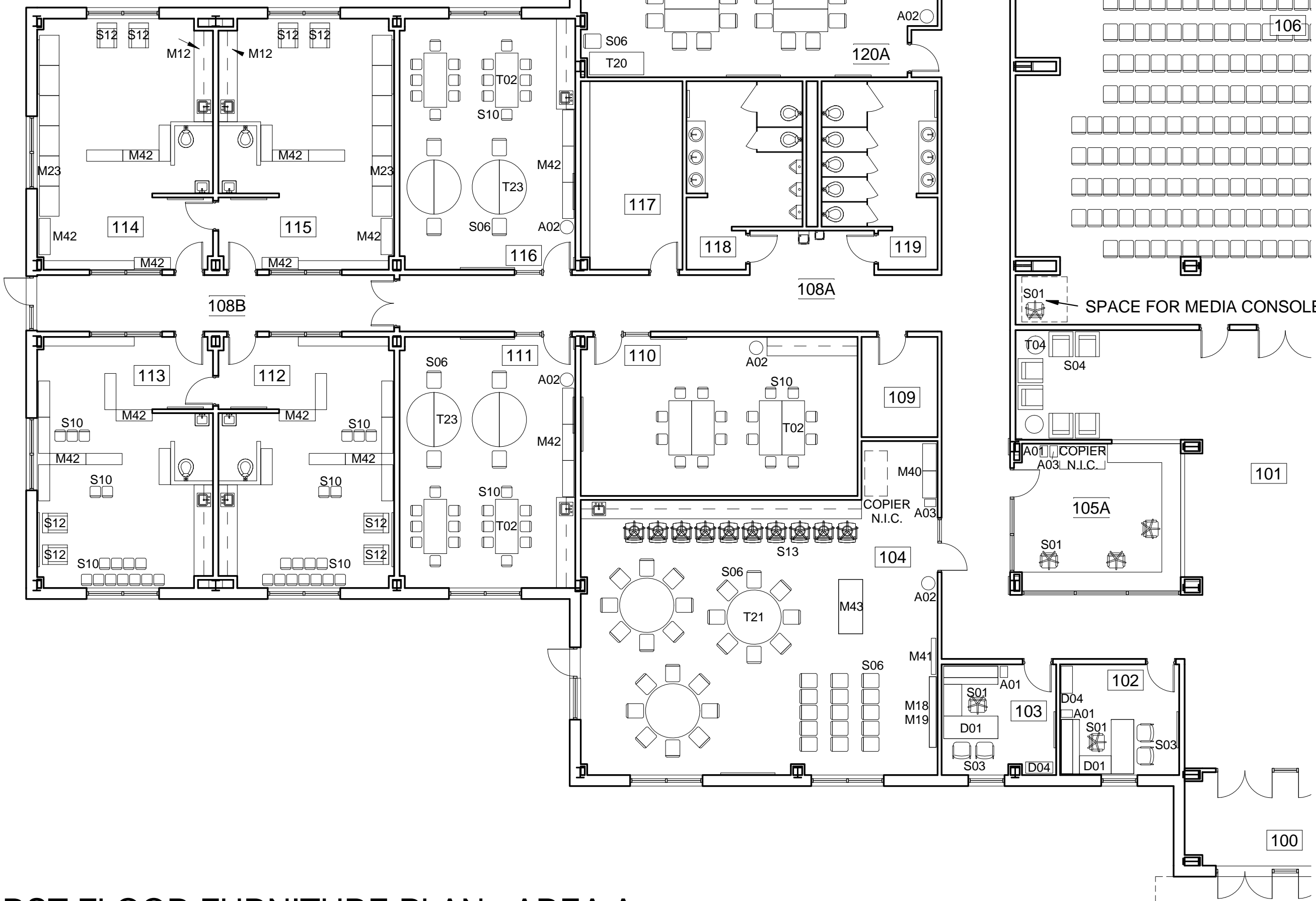
FIRST FLOOR FURNITURE PLAN - AREA A
