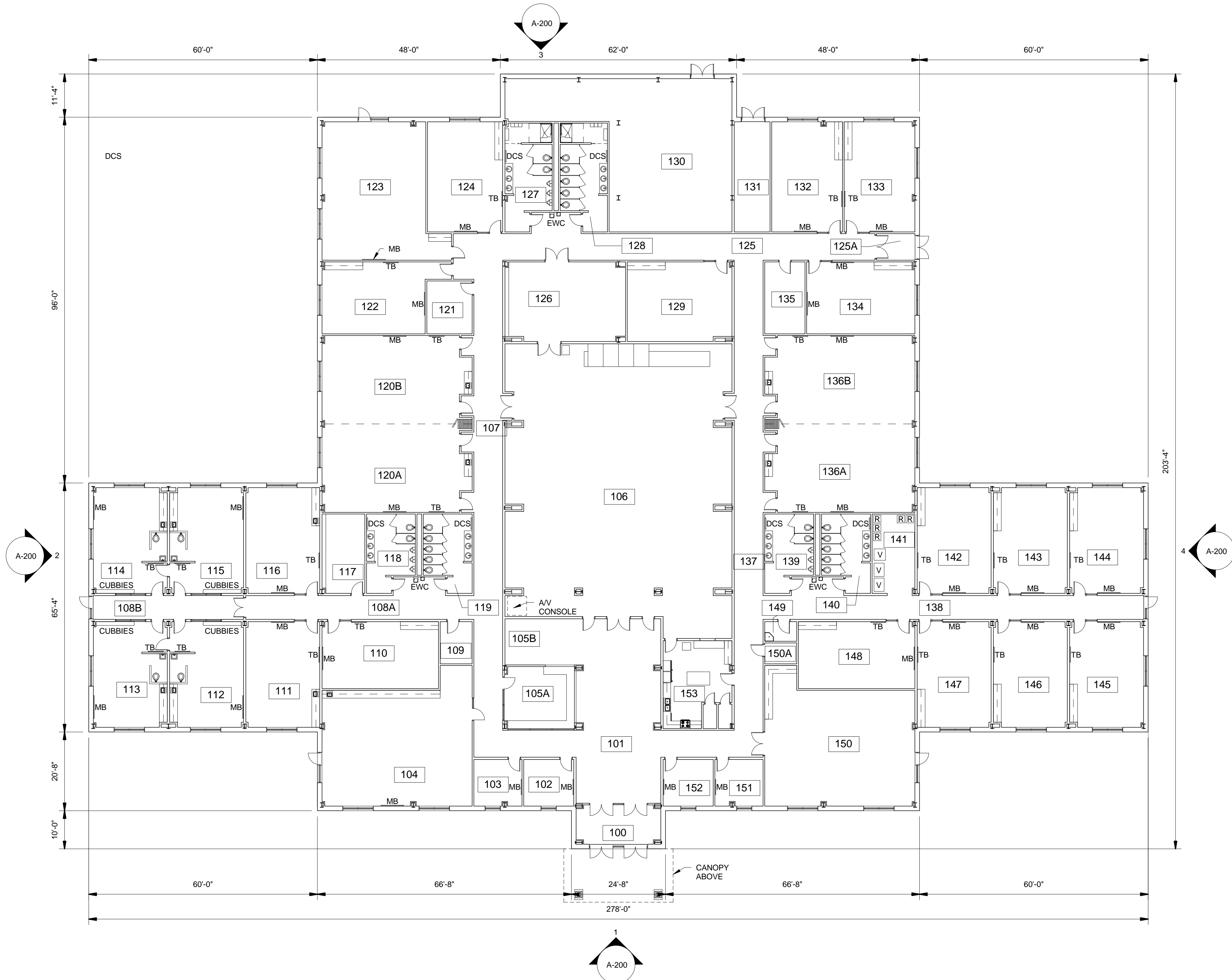
1 A-110 COMPOSITE FIRST FLOOR PLAN 1/16" = 1'-0"
