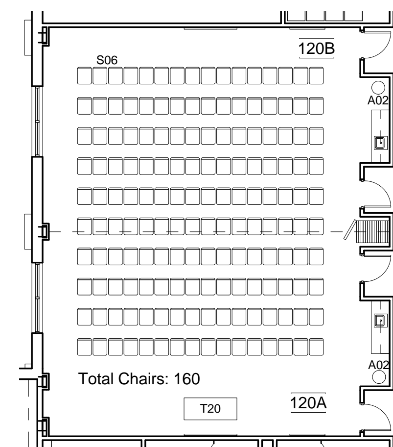
1 LARGE CLASSROOM ALTERNATE LAYOUT
