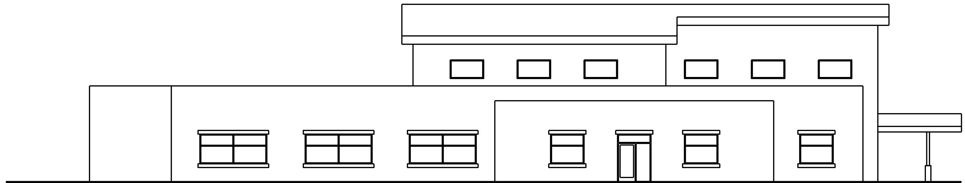
2 BUILDING ELEVATION A-100 3/32" = 1' 0"
