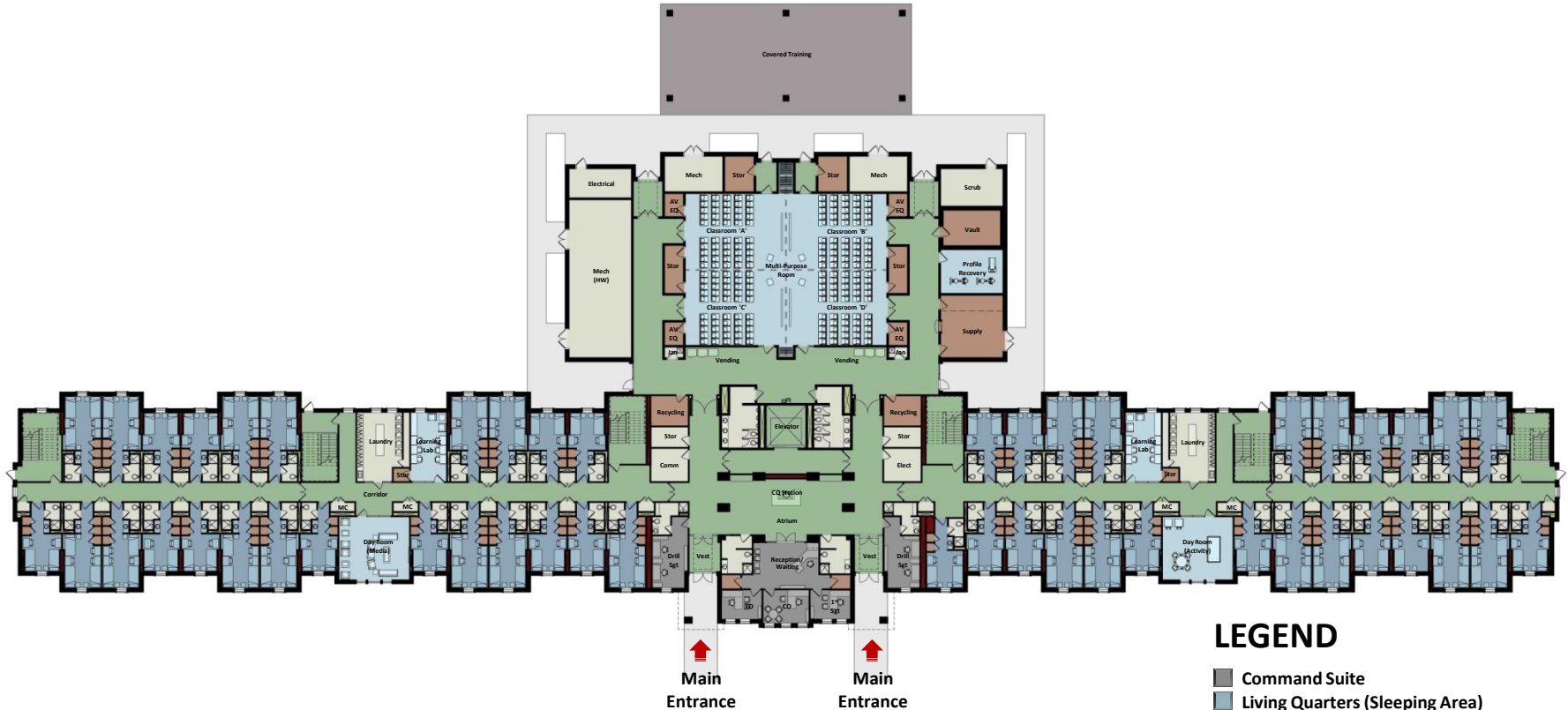
Conceptual Floor Plan (First Floor)
