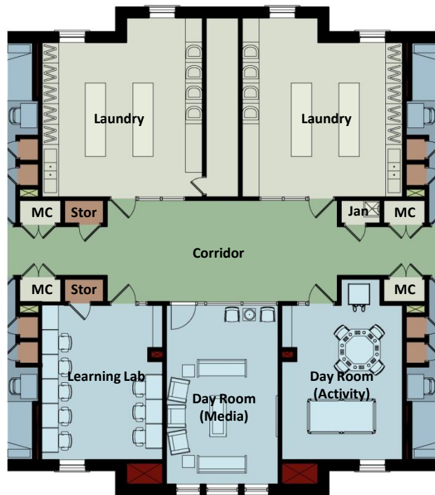
Training Support Module 'A'
