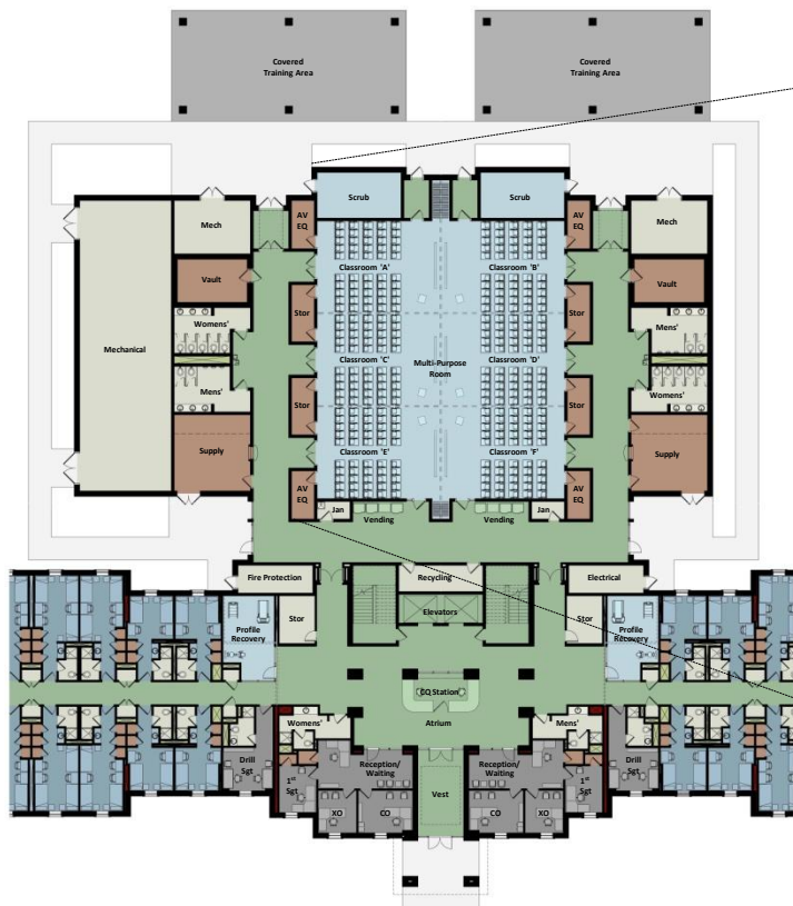
Partial Floor Plan - Core Area (First Floor)
