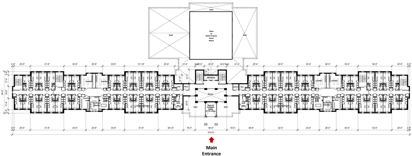
Conceptual Floor Plan (Second thru Fifth Floors) No Scale
