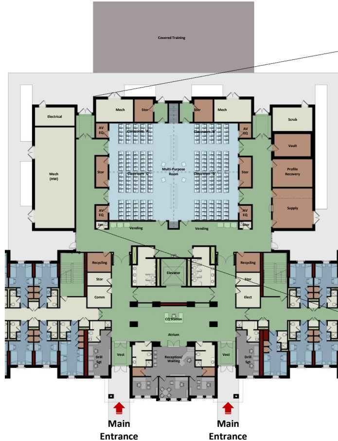
Partial Floor Plan - Core Area (First Floor)
