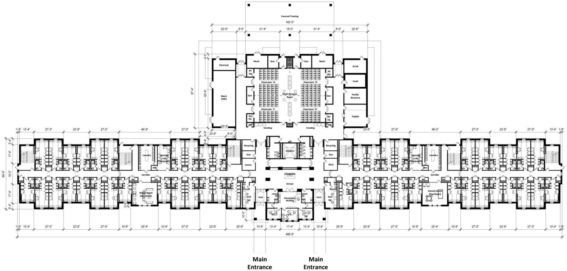
Conceptual Floor Plan (First Floor)
