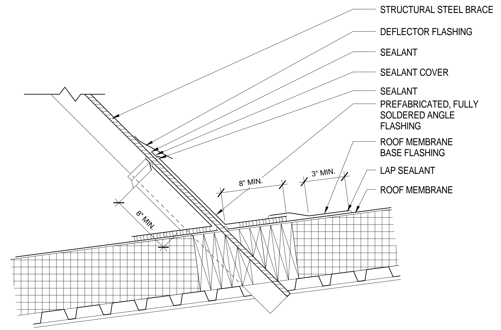
5 STRUCTURE PENETRATION 1 1/2" = 1'-0"
