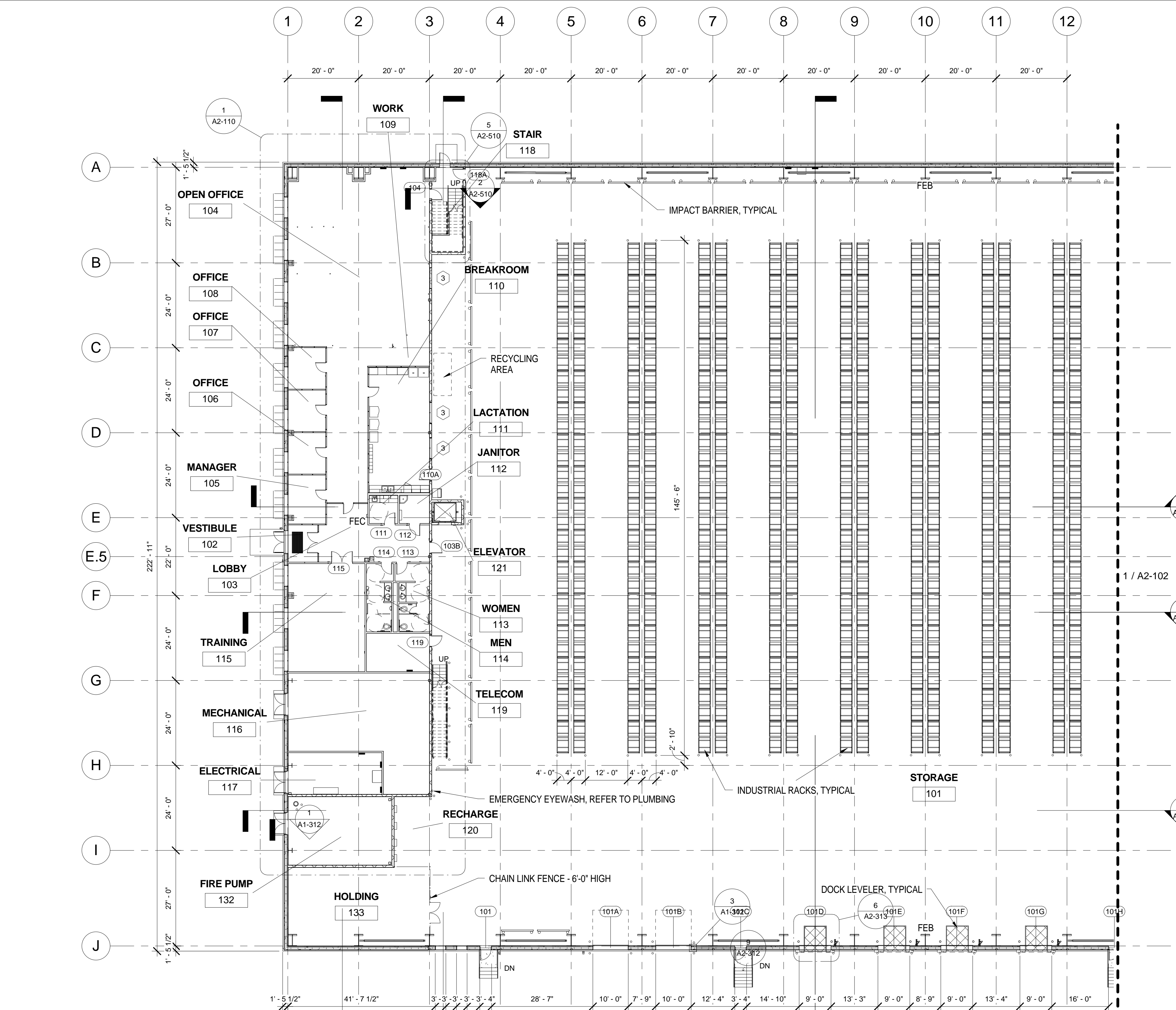
PLAN NORTH PARTIAL FLOOR PLAN - AREA 1 1/16" = 1'-0" SCALE: 1/16" = 1'-0" 16' 0 16' 32'
