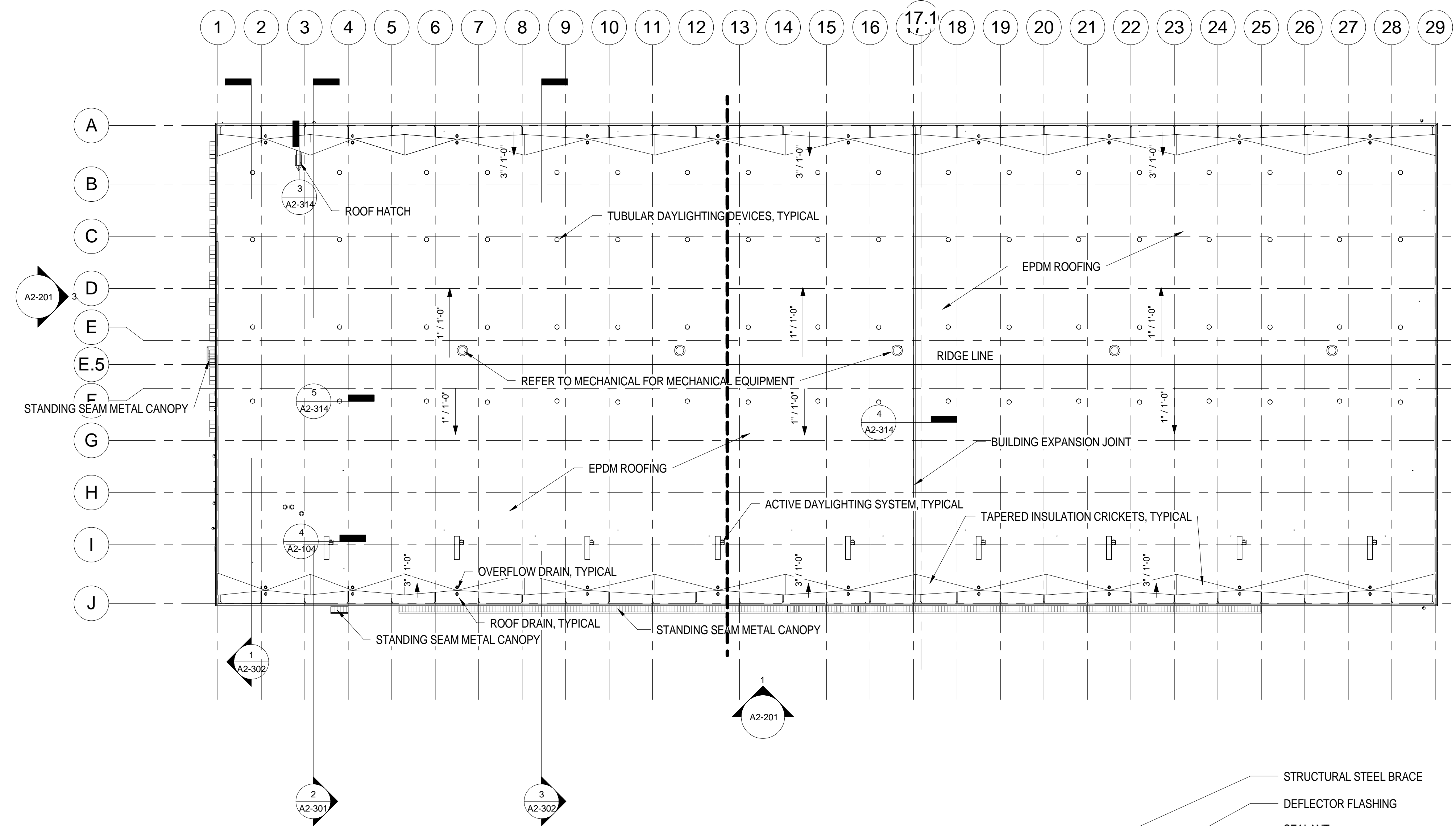
PLAN NORTH 1 ROOF PLAN 1/32" = 1'-0"
