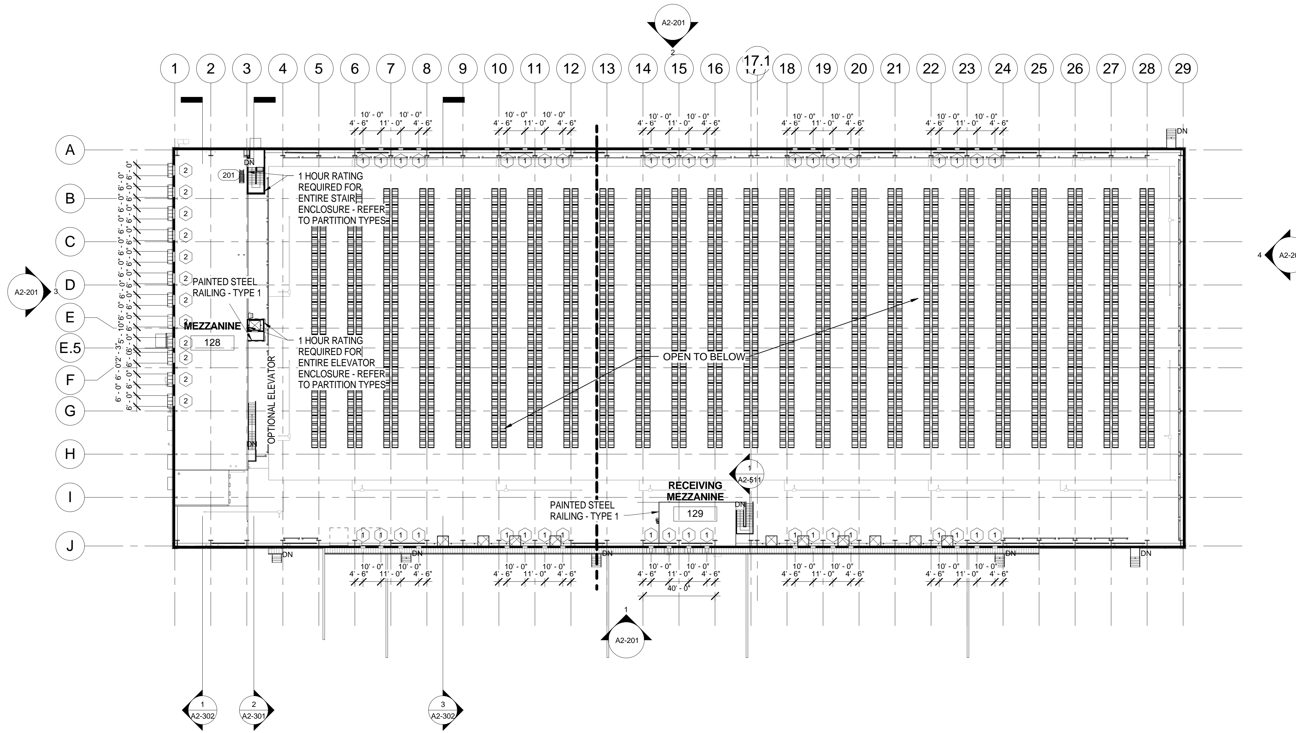
1 A2-103 1/32" = 1'-0" MEZZANINE PLAN
