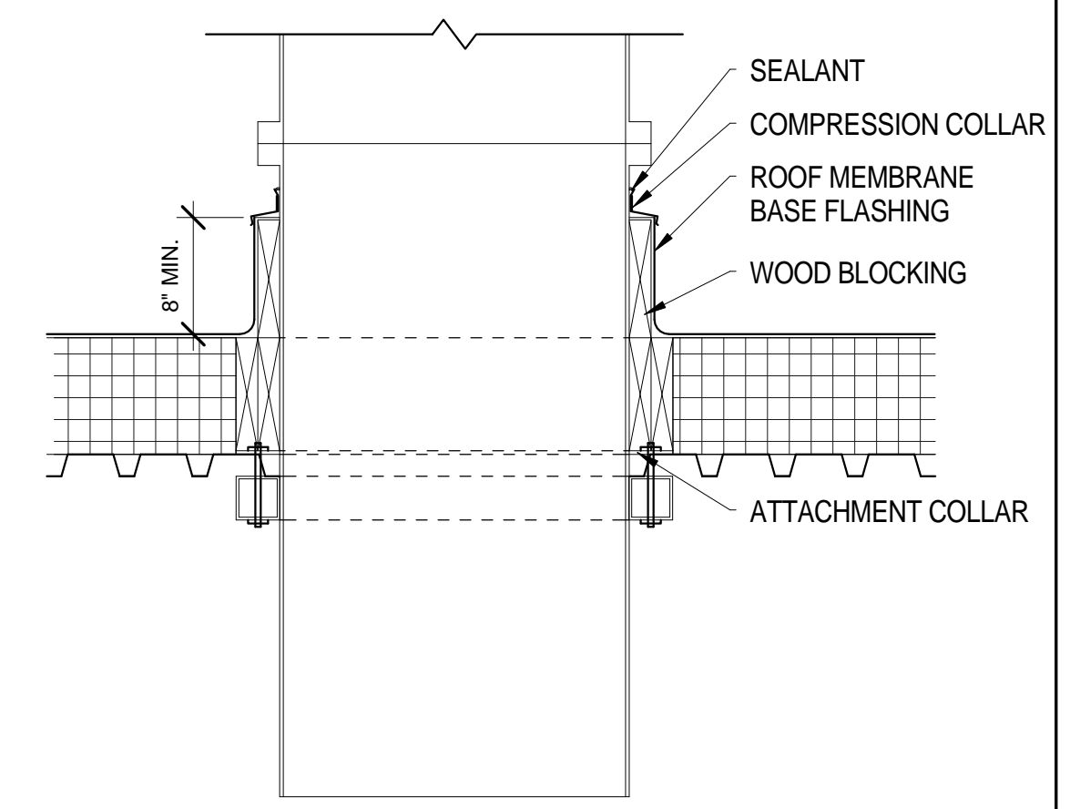
4 ACTIVE DAYLIGHTING SYSTEM 1" = 1'-0"
