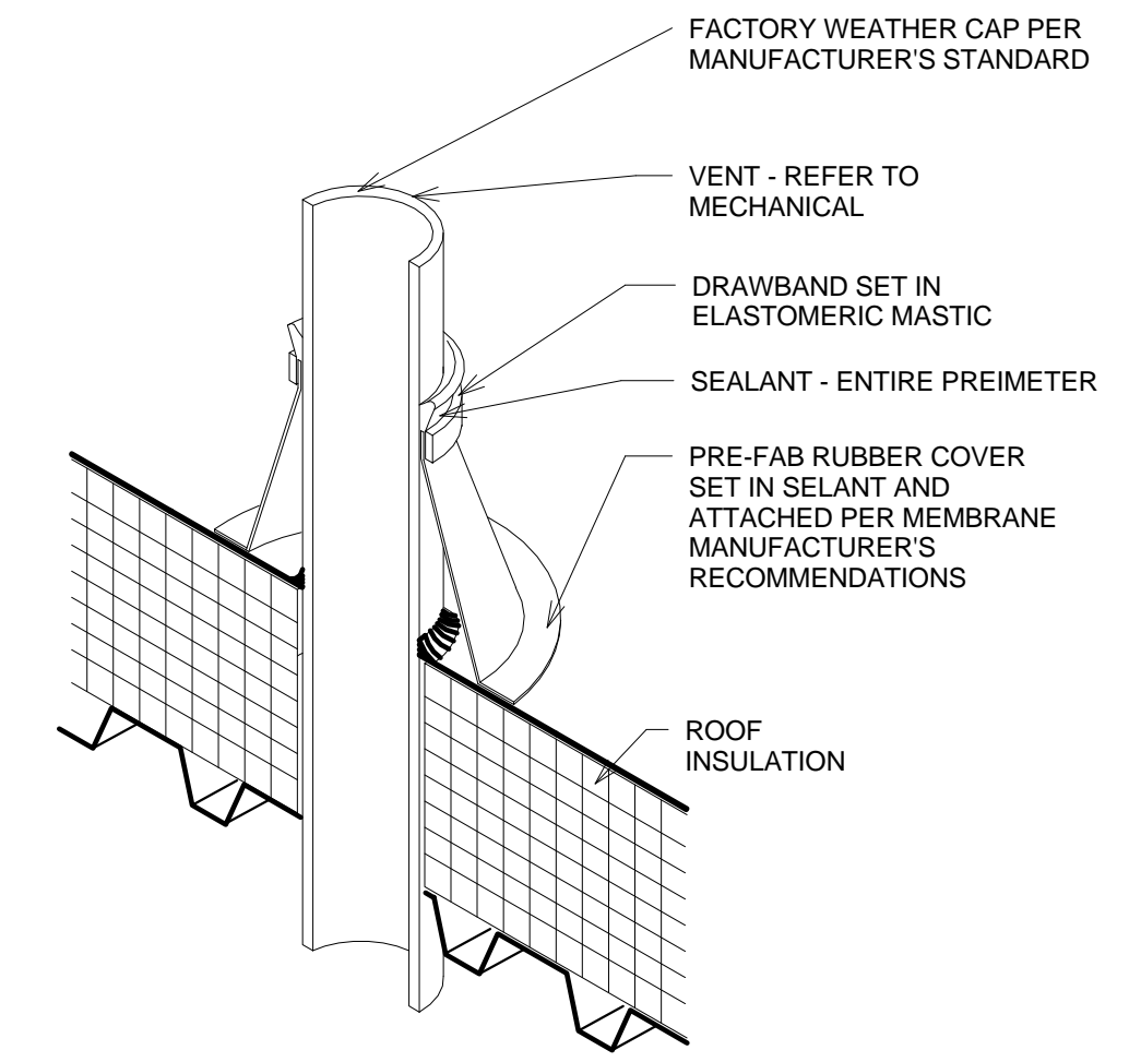
2 TYPICAL ROOF PENETRATION 1 1/2" = 1'-0"
