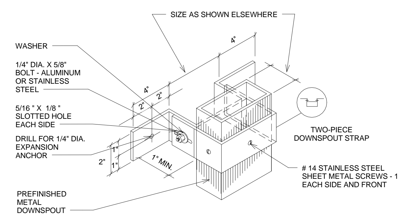
3 DOWNSPOUT 3" = 1'-0"
